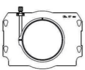
Clamp Adapter K2.47240.0 (ø 114 mm)
