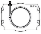
Clamp Adapter K2.47253.0 (ø 104 mm)
